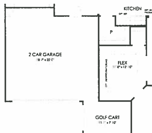
Golf Cart Bay (Not Available with 4ft Garage Extension)
